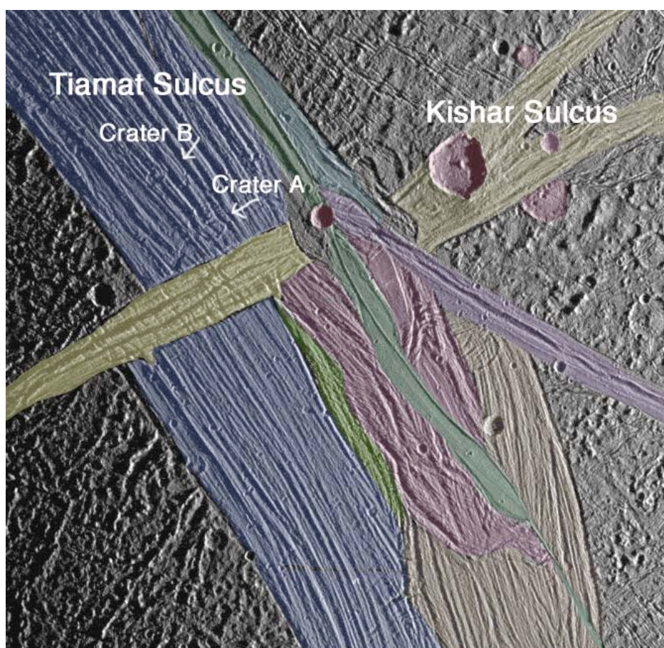
Figure 2: Tiamat and Kishar Sulcus, imaged at 494 meters/pixel during Galileo's 28 th orbit. North is up.
